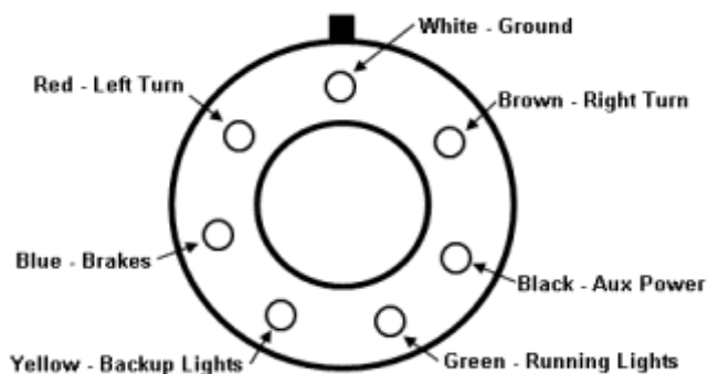
Figure 1 Looking into the Vehicle Socket
